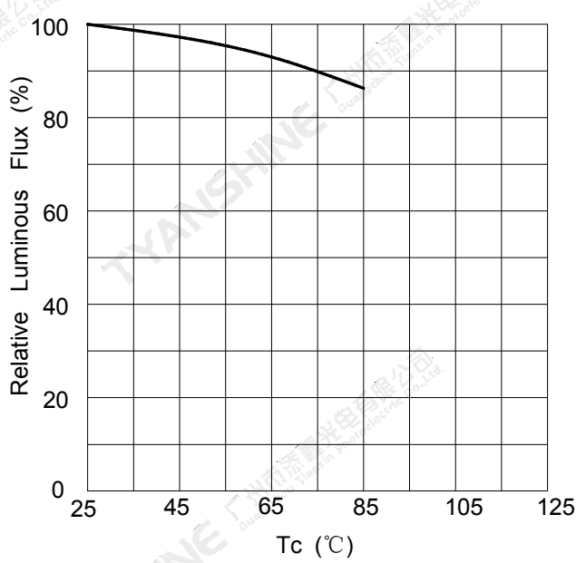
Temperature VS. Relative Luminous Flux (IF=3.2A)
