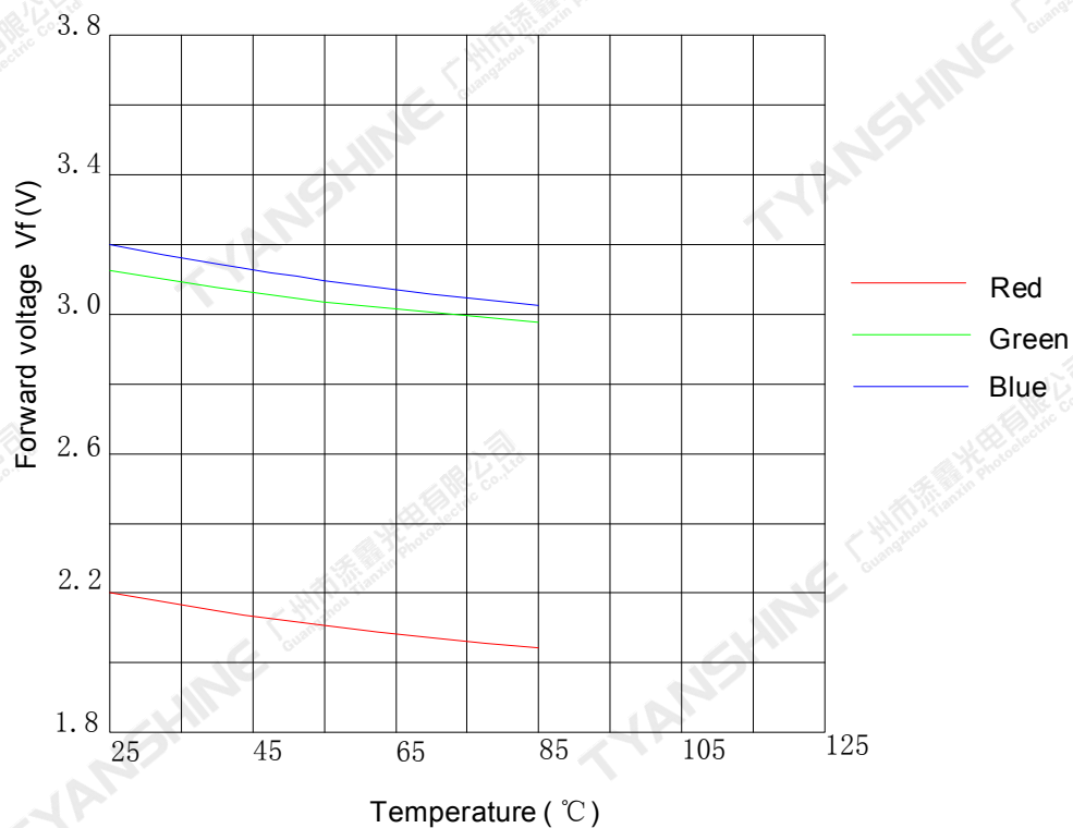
Temperature VS. Forward Voltage (IF=160mA)
