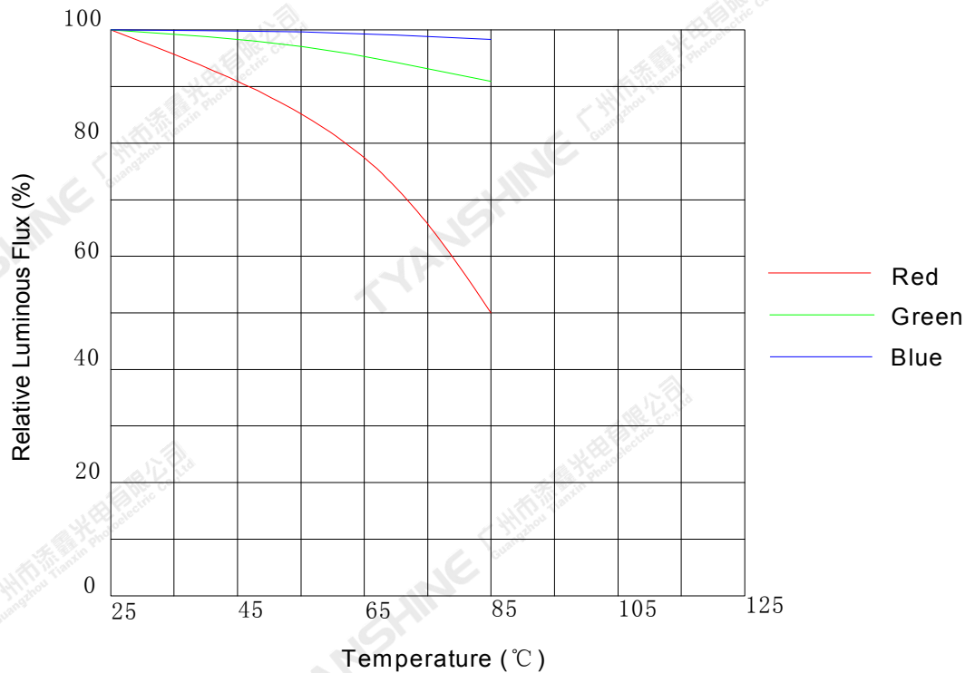
Temperature VS. Relative Luminous Flux (IF=160mA)
