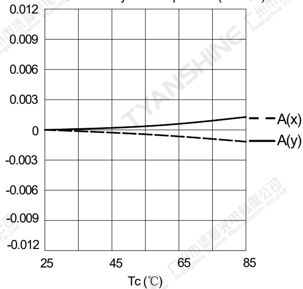
Relative Chromaticity VS. Temperature (IF=1.0A)
