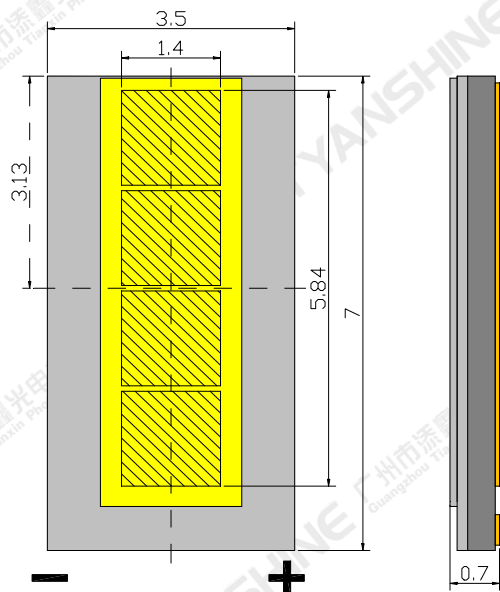
Top view
