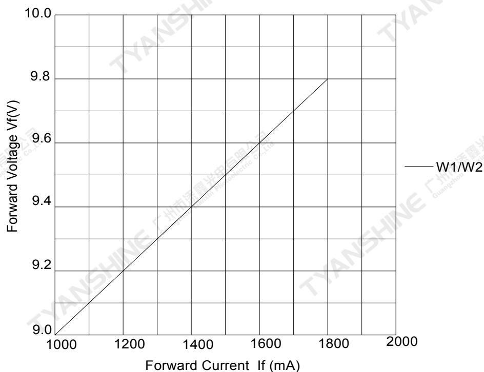
Forward Current VS. Forward Voltage
