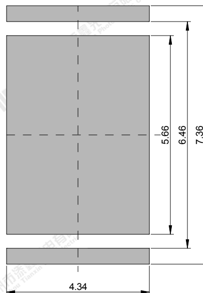
recommended stencil pattern
