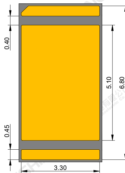
Bottom view
